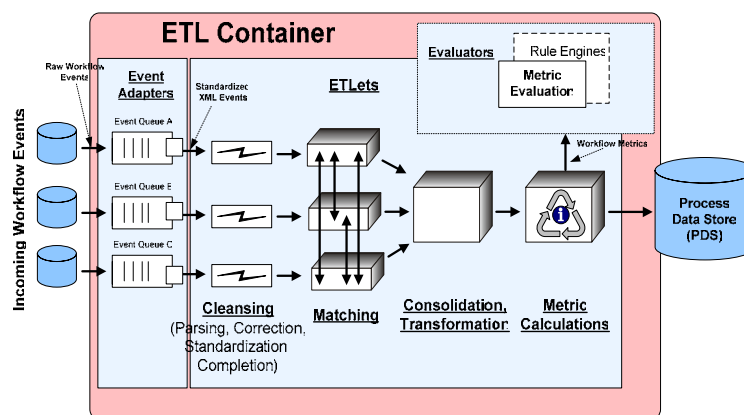
Figure 2: ETL Container – Architecture [1]
