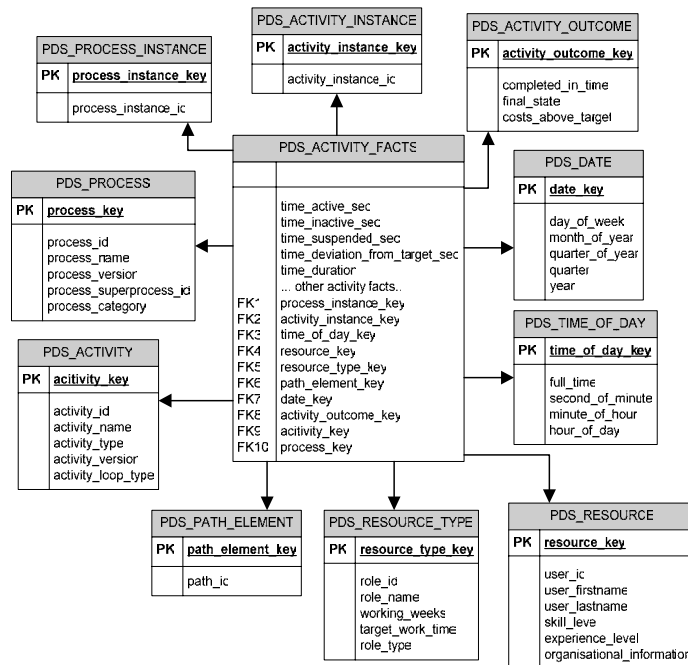
Figure 3: Activity-Level Facts of the PDS
