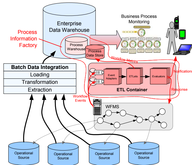
Figure 1: Process Information Factory with Process Data Store
